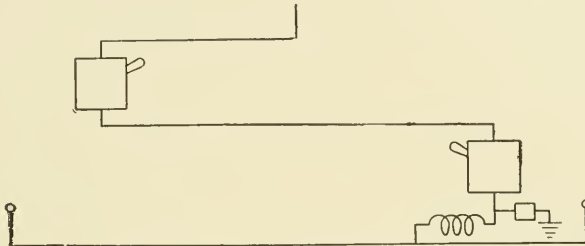
Fig. 127. Diagram of Series Connections for Hand-Operated Circuit Breakers
